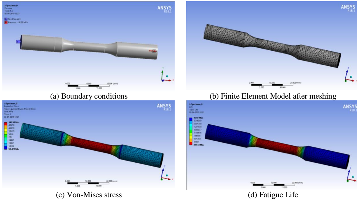
Figure 4: FE Analysis of specimen without notch
