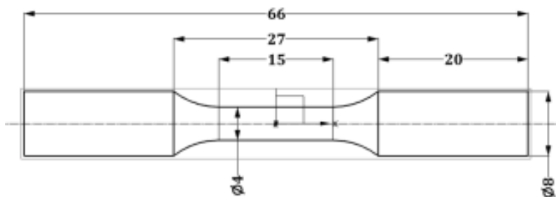
Figure 2: Drawing of the specimen
