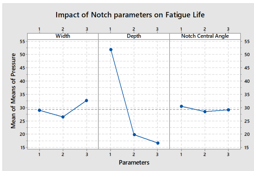
Figure 6: Variation of Pressure w.r.t. the parameters
