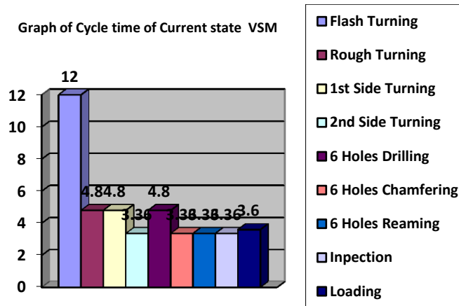
Fig 5. Graphical Representation of Current state VSM.
