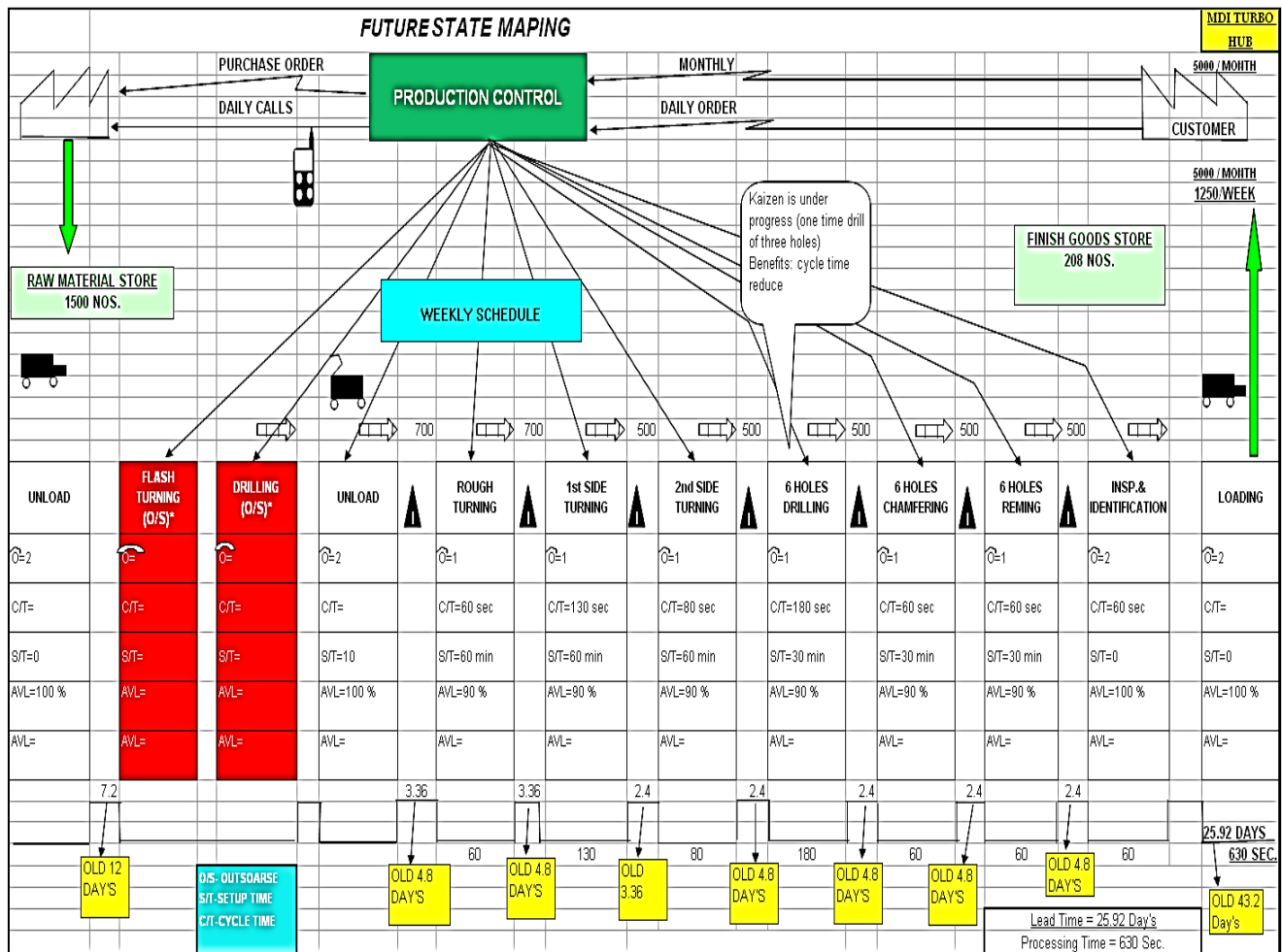
Fig 6. Future Value Stream (V.M. Auto Pvt. Ltd.)
