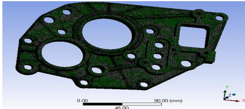
Fig 2-Finite Element model
