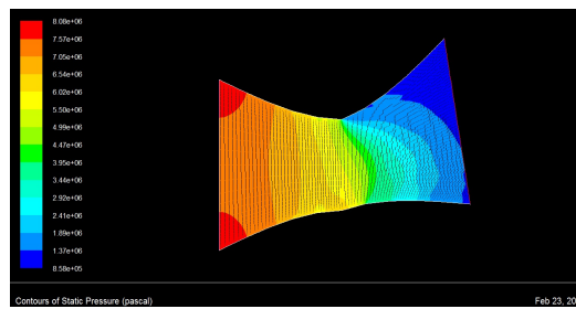
Fig. 8. Pressure contour of c-d nozzle ( \theta=20 )
