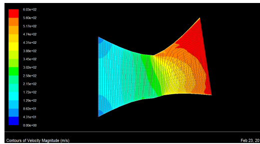
Fig. 9. Velocity contour of c-d nozzle ( \theta=20 )
