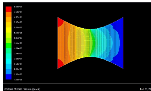
Fig. 4. Pressure contour of c-d nozzle ( \theta=0 )
