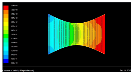
Fig. 5. Velocity contour of c-d nozzle ( \theta=0 )
