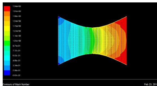
Fig. 10. Mach no contour of c-d nozzle ( \theta=0 )
