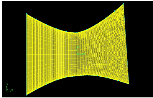
Fig. 2. Geometry of c-d nozzle ( \theta=10 )
