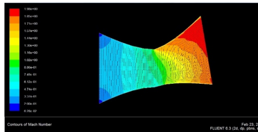
Fig. 12.Mach no contour of c-d nozzle ( \theta=20 )
