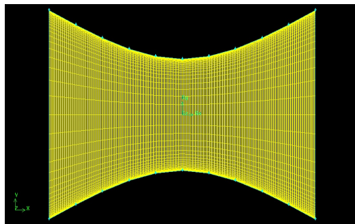
Fig. 1. Geometry of c-d nozzle ( \theta=0 )
