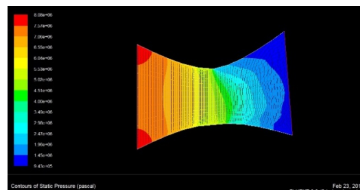
Fig. 6. Pressure contour of c-d nozzle ( \theta=10 )
