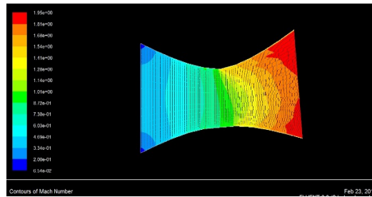
Fig. 11.Mach no contour of c-d nozzle ( \theta=10 )
