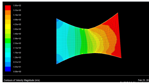
Fig. 7. Velocity contour of c-d nozzle ( \theta=10 )
