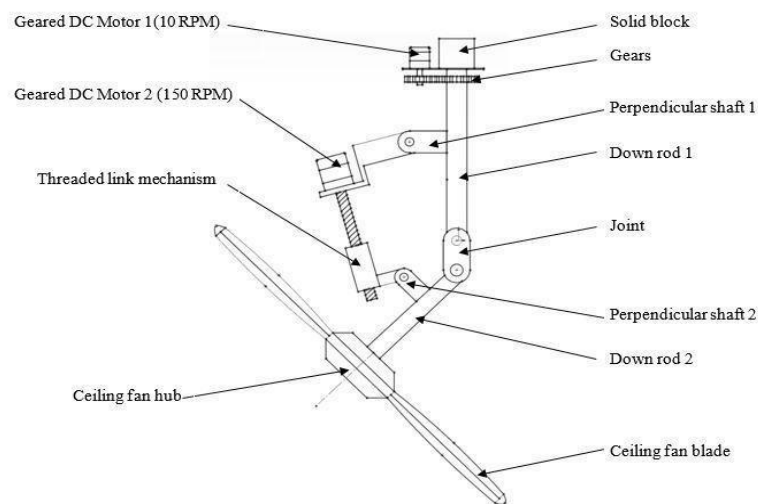
Fig.2 Custom Angle Ceiling Fan
