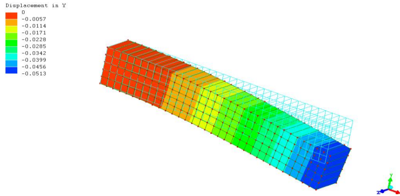
Fig 9 - Displacement of beam without hole
