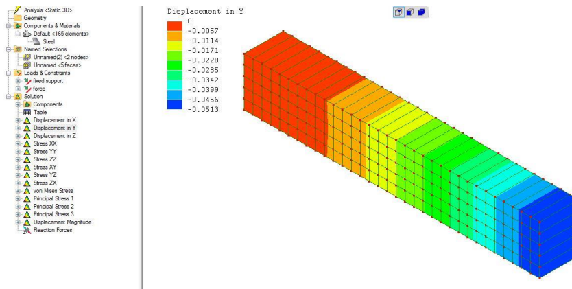
Fig 8- Results are listed below solution
