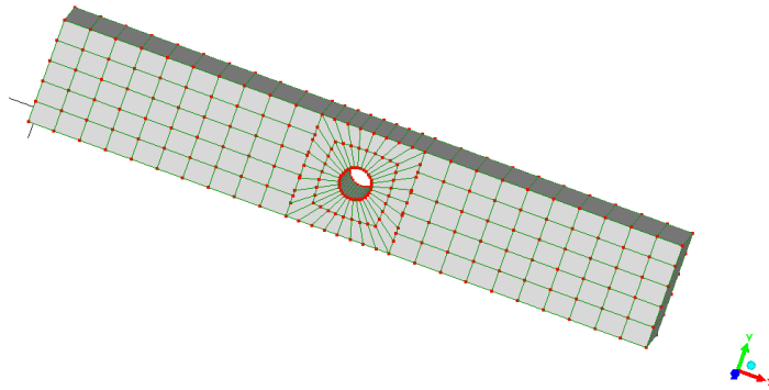
Fig 5 – Circular Hole In Beam
